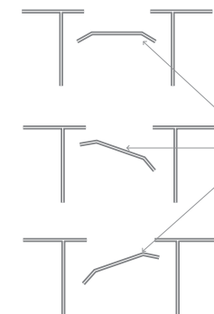
FIGURE 1 ADJUSTABLE AIR FLOW DIVERTER
